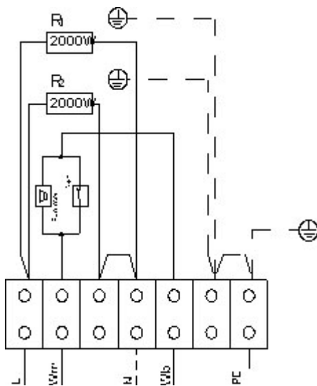
Connection circuitbreaker device
