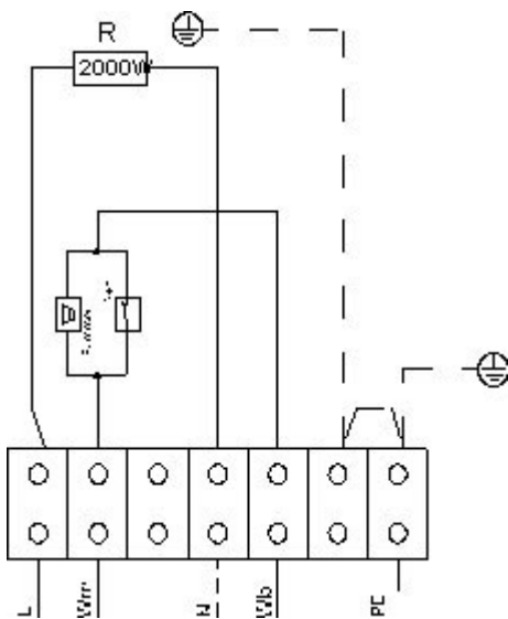
Connection control panel
